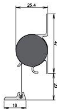
FP200 Dimensions
