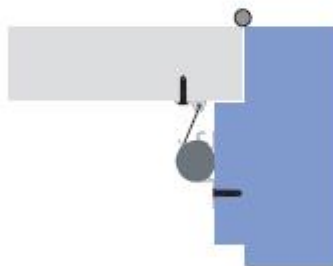
FP200 Application
